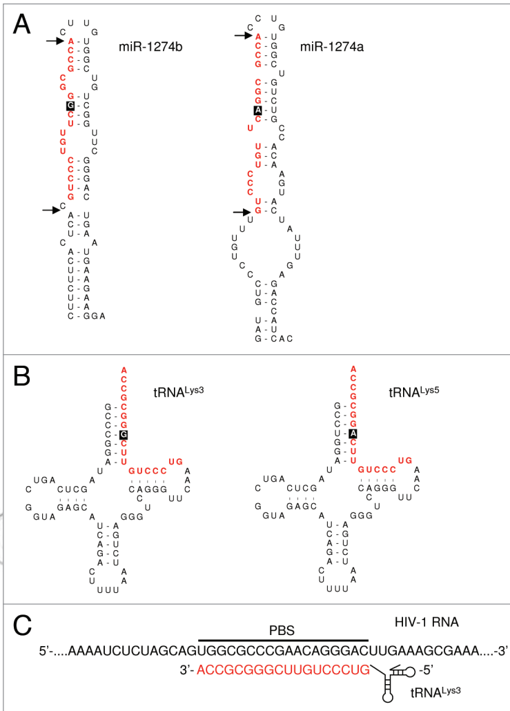
Figure 1. Mature human miR-1274a and miR-1274b are tRNA Lys mimics. (A) The predicted secondary structure of the miR-1274b and 1274a stem loop structure. Dicer cleavage sites are indicated by arrows and the mature miRNA sequence is marked in red. The single nucleotide difference between the mature miR-1274b and 1274a is shown as black boxed nucleotide. (B) The cloverleaf secondary structure of tRNA Lys3 and tRNA Lys5 , indicated in red is the sequence that mimics the proposed miRNAs and that was found by deep sequencing. The nucleotides in the black box indicate a single nucleotide difference between the two tRNAs, similar to the mature miRNAs. (C) Both tRNA Lys molecules are used as primer in HIV-1 RNA reverse transcription. The priming of reverse transcription by tRNA Lys3 is depicted. The 3' end of the tRNA Lys3 (red sequence) binds to the primer binding site (PBS) of HIV-1 RNA and the 3'-OH is subsequently extended.
