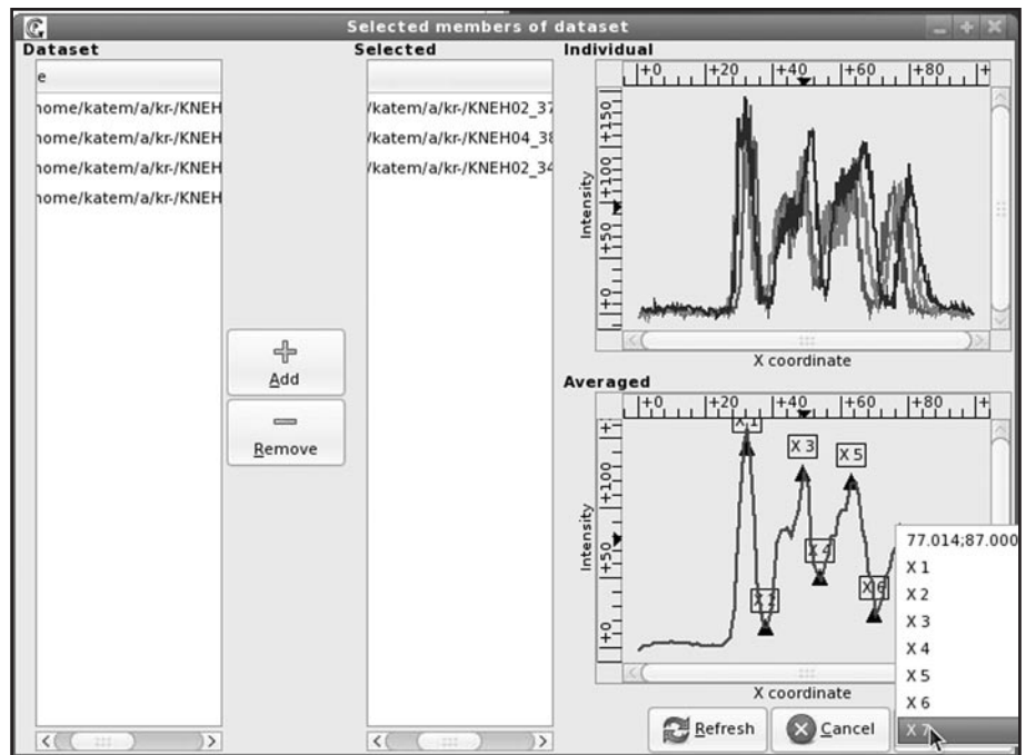
Figure 2. GUI for extraction of the GCP template. The template is constructed for eve expression pattern in embryos mutant for Kr belonging to late cycle 14A (time class 6 according to our classification, see Materials and methods). The Dataset panel (left) shows the folders containing the dataset. Any number of files can be selected and moved to the Selected panel by pressing the Add button. The upper panel on the right (Individual) presents the graphs of selected patterns; while in the lower panel (Averaged) the average of these patterns is plotted. The pop-up menu shows cursor coordinates and the list of feasible GCPs.
