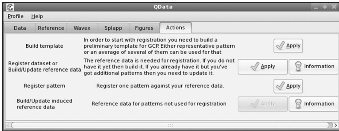
Figure 1. GCPReg interface.
