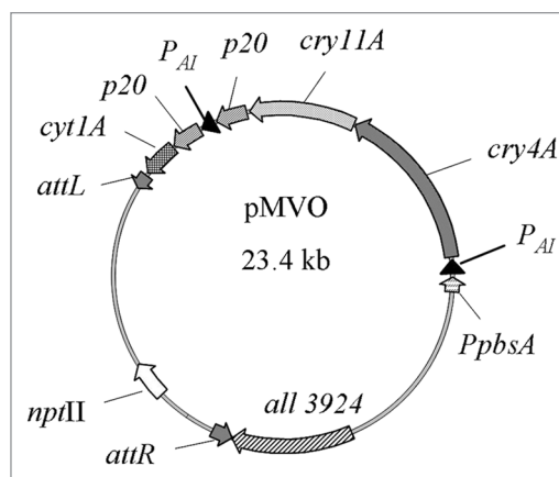
Figure 2. Plasmid pMVO, designed for excision by Int via site-specific recombination between the attR and attL sites. The 23.4 kb pMVO carries the four Bt toxin genes ( cry4A , cry11A , p20 [twice] and cyt1A ) and antibiotic resistance marker nptII . Two promoters were introduced, P_{psbA} (of the photosystem II's D1) and P_{A1} (T7 phage early promoter) at the denoted positions. nptII , neomycin/kanamycin resistance gene; ORF all3924 , a PCR amplified sequence 24 encoding a probable penicillin amidase (see in http://bacteria.kazusa.or.jp/cyanobase/index.html ).
